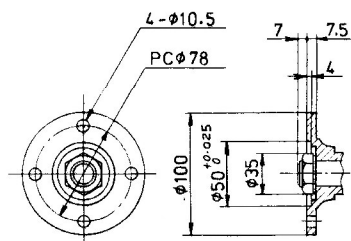
DETAIL OF COUPLING (A) (SCALE 1/3)
