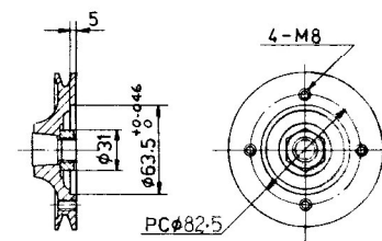
DETAIL OF PULLEY (B) (SCALE 1/3)
